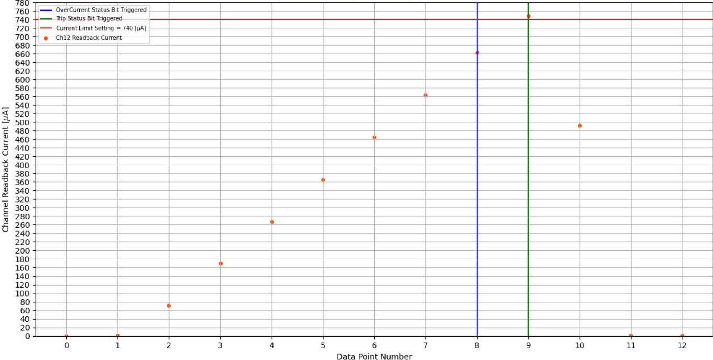
Module 353, Slot 0, Channel 12 Trip Test
