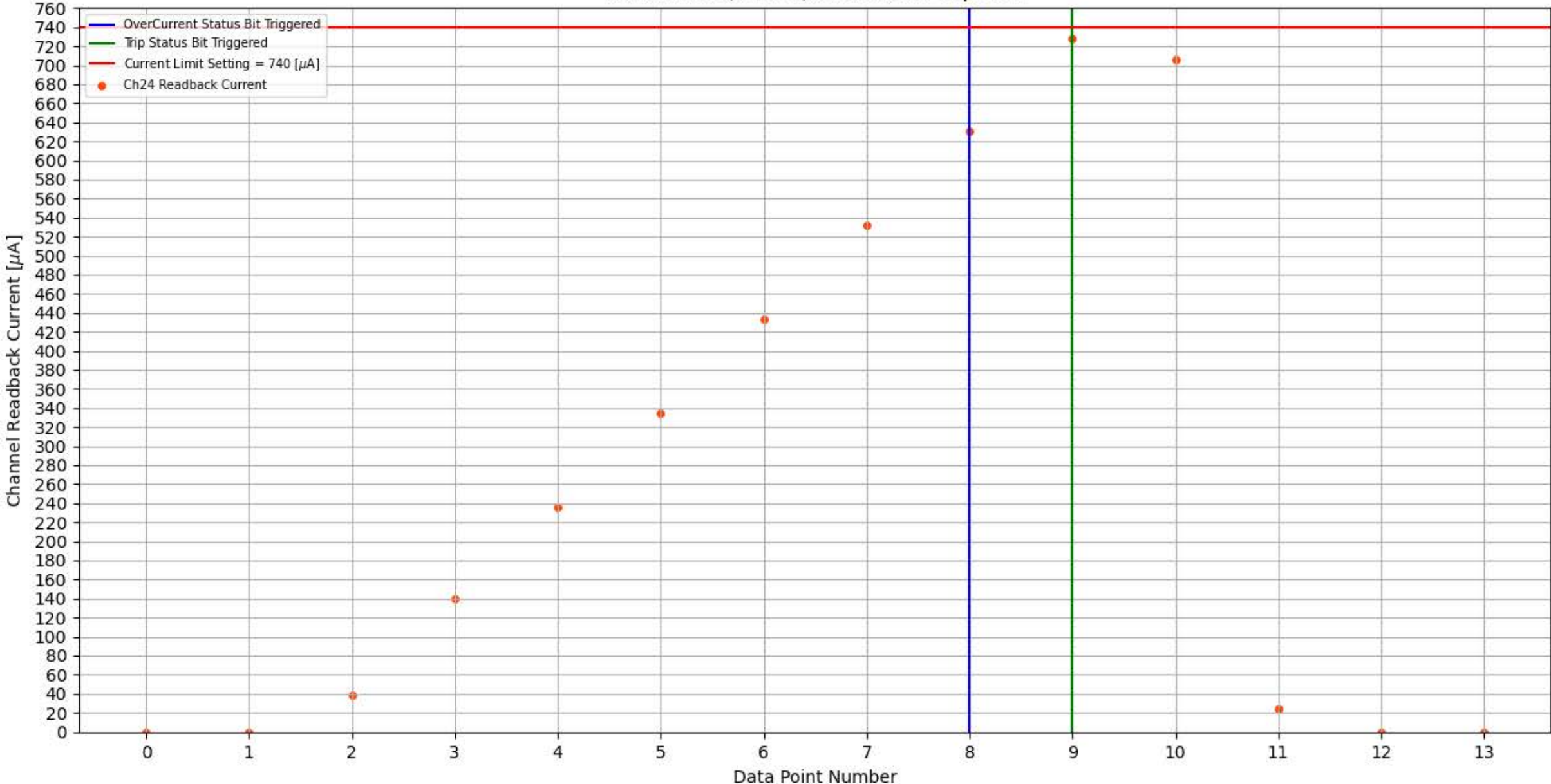
Module 353, Slot 0, Channel 24 Trip Test
