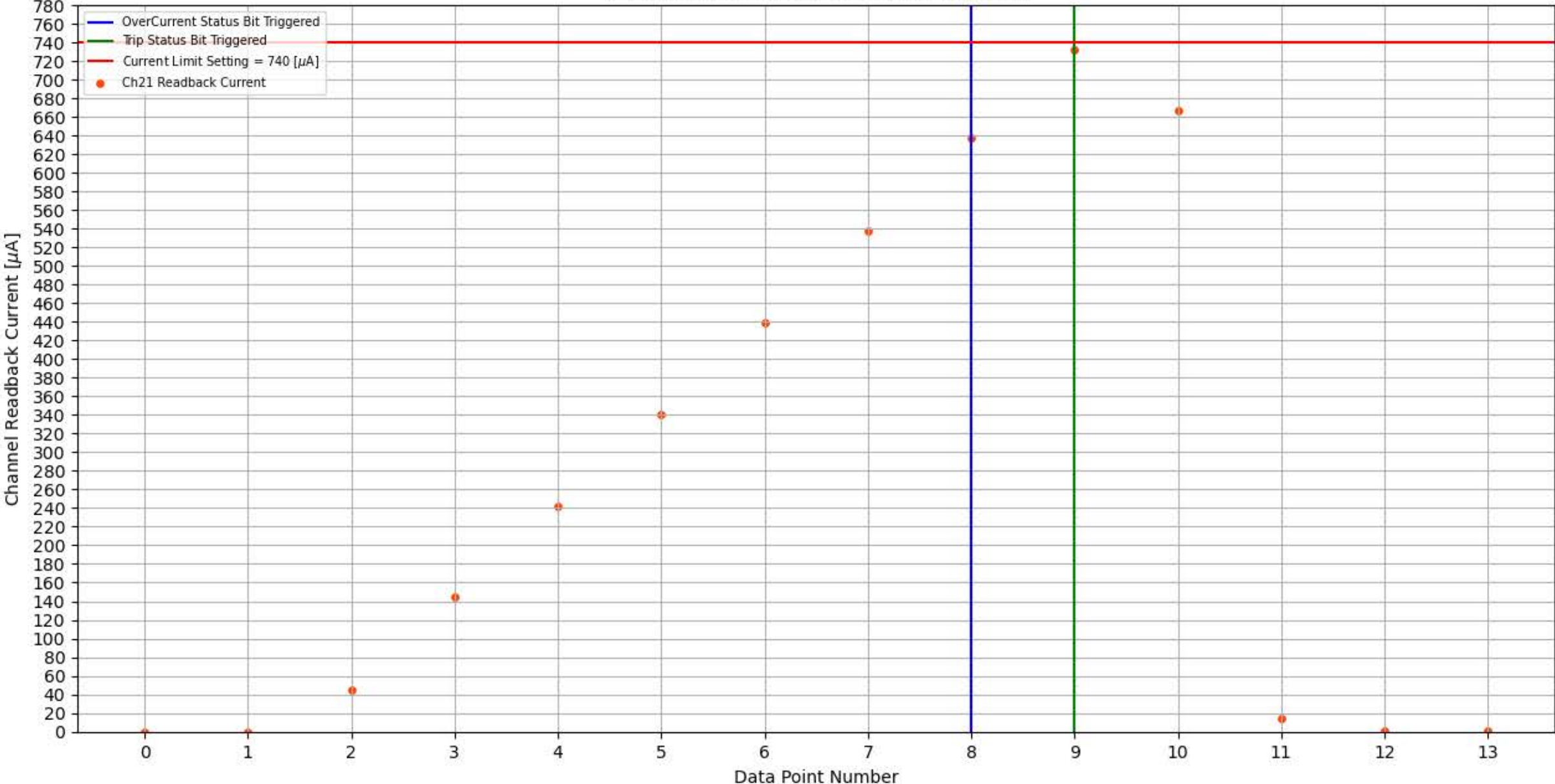
Module 353, Slot 0, Channel 21 Trip Test
