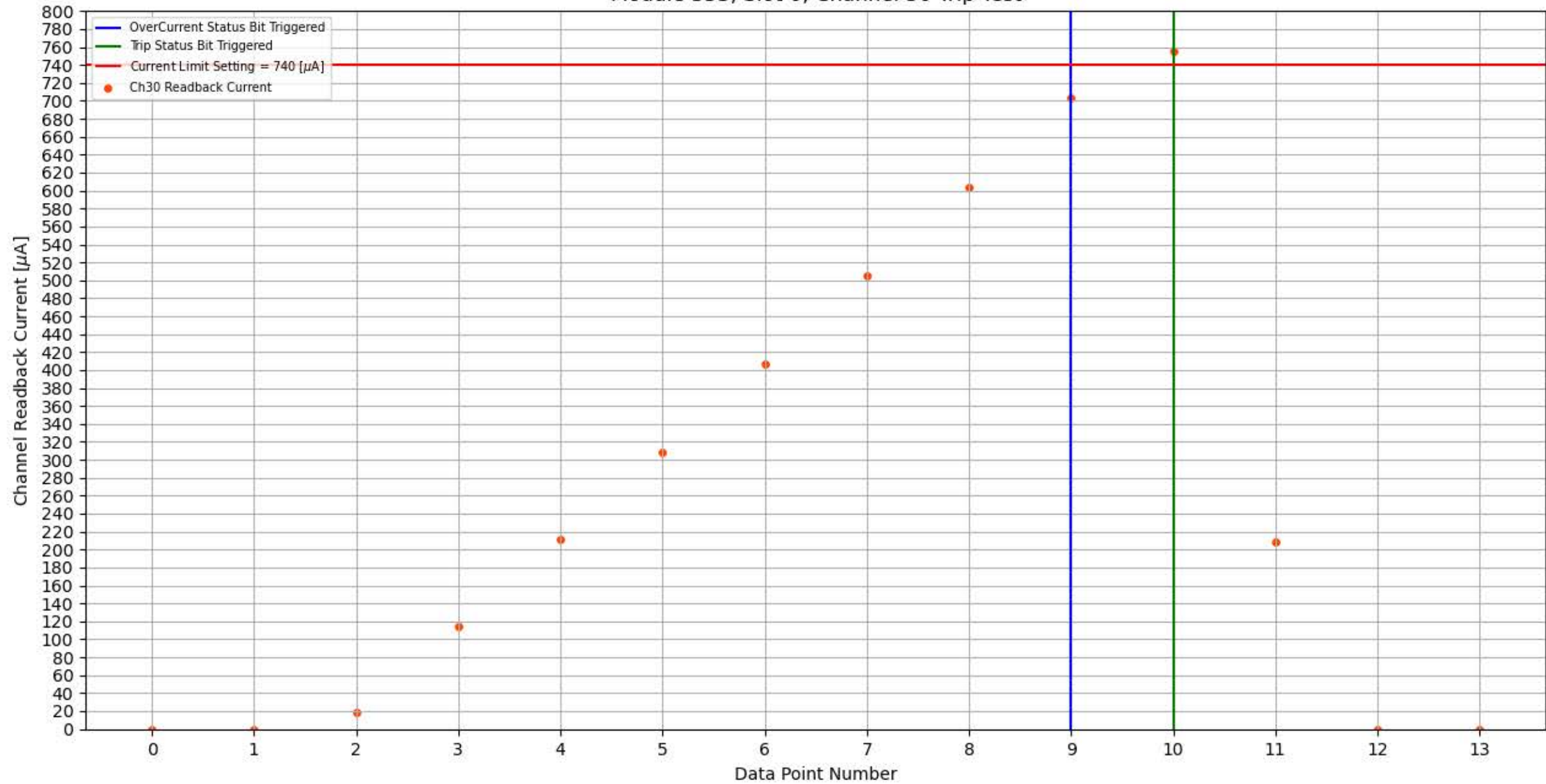
Module 353, Slot 0, Channel 30 Trip Test
