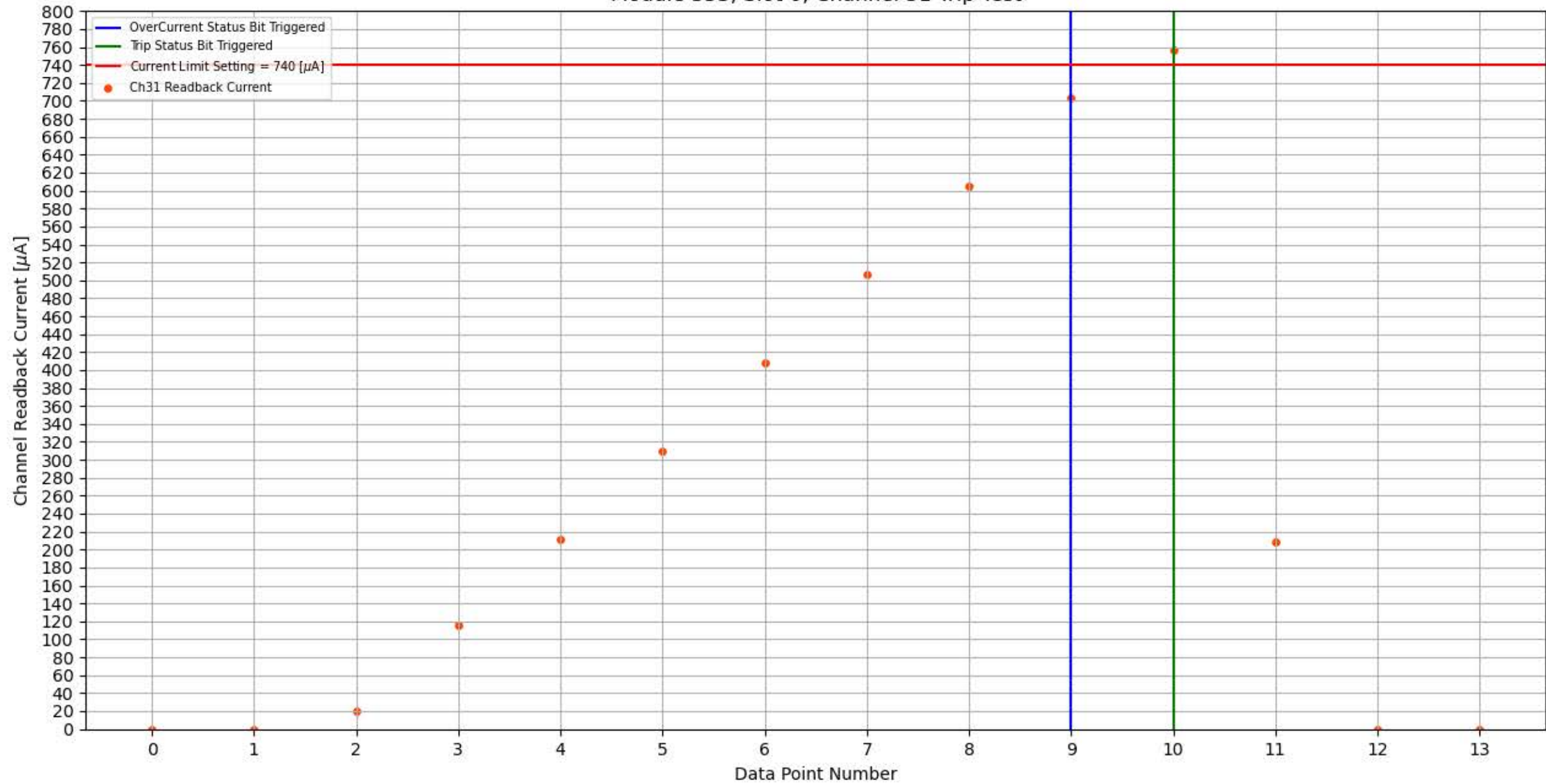
Module 353, Slot 0, Channel 31 Trip Test
