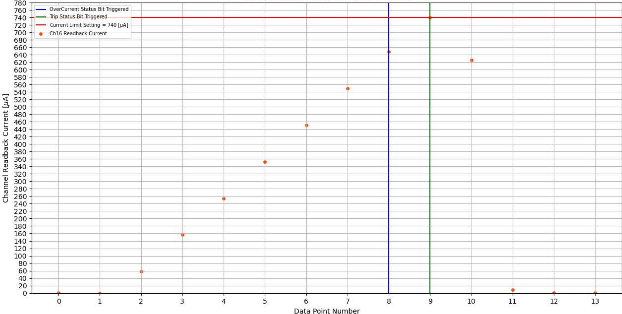
Module 353, Slot 0, Channel 16 Trip Test
