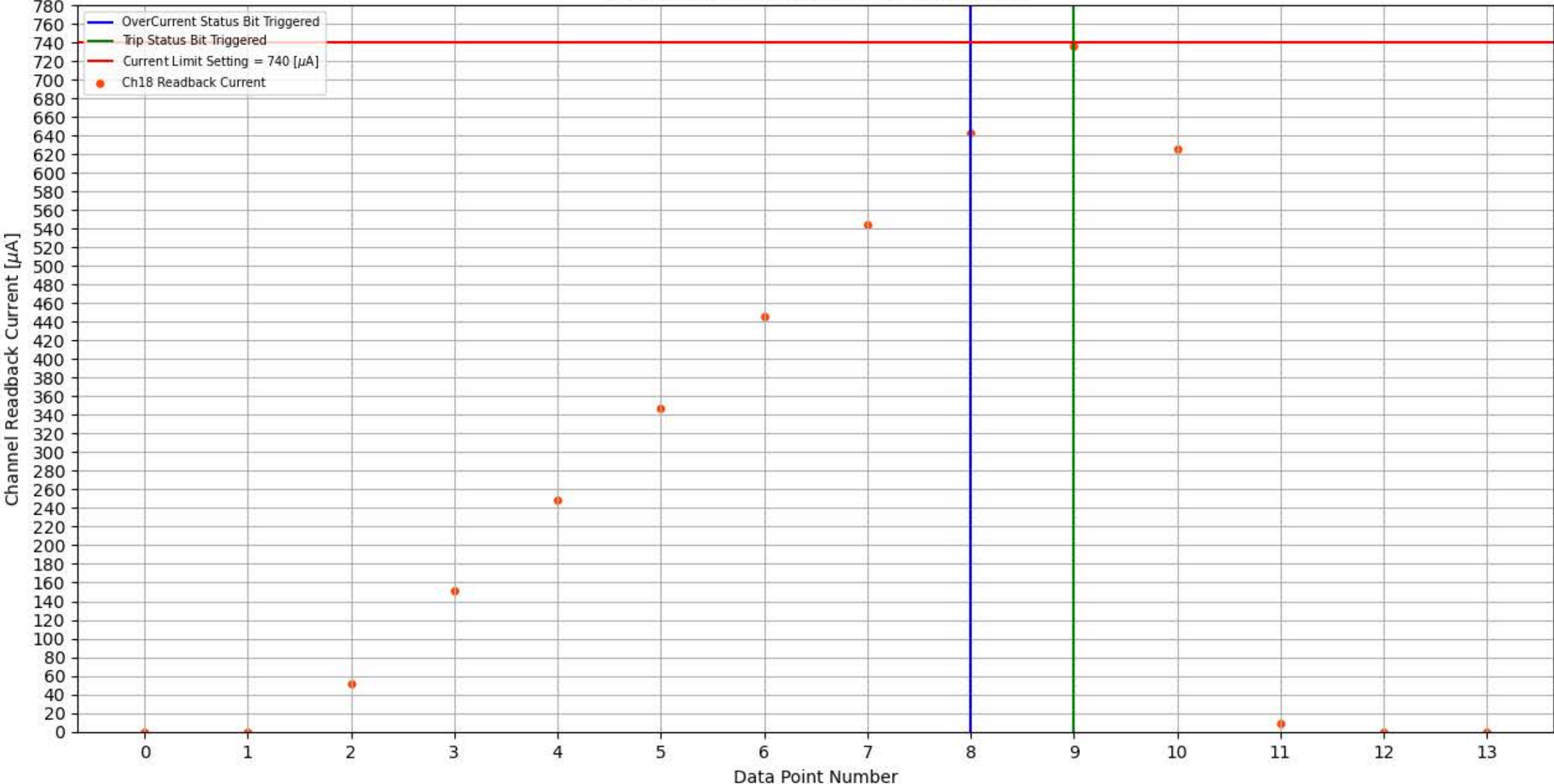
Module 353, Slot 0, Channel 18 Trip Test
