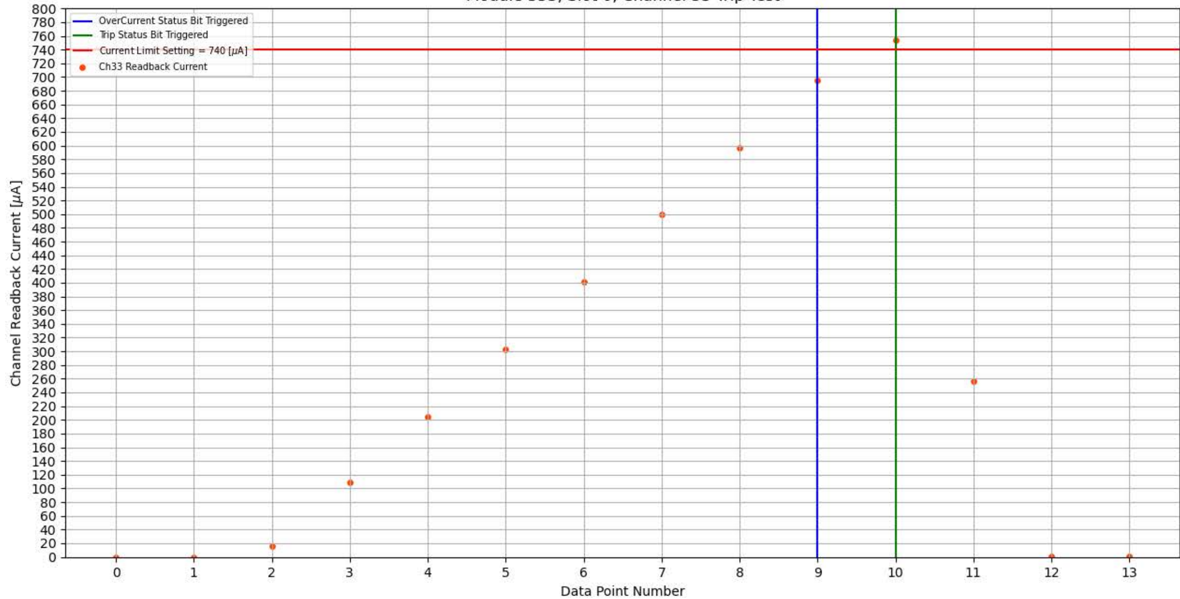
Module 353, Slot 0, Channel 33 Trip Test
