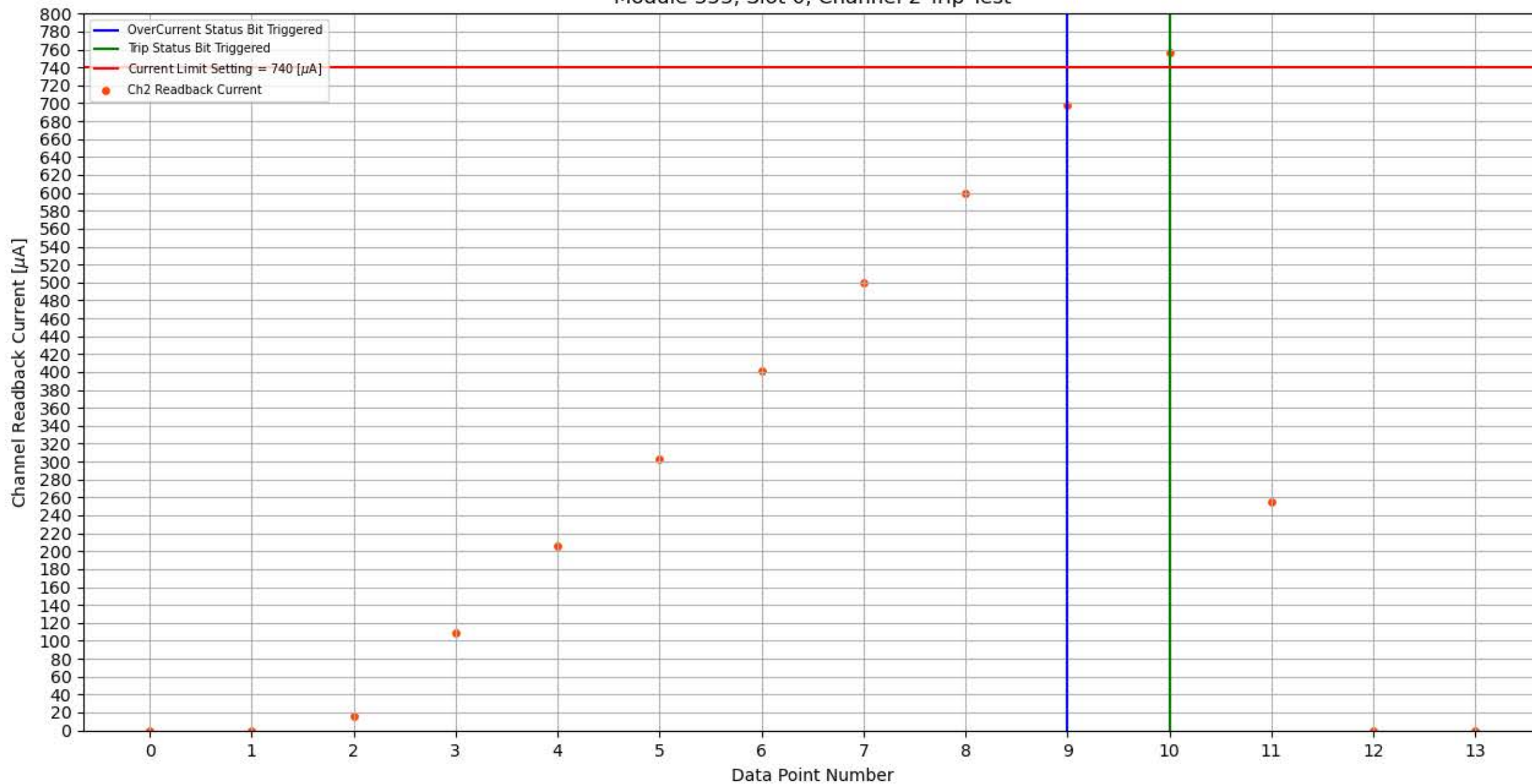
Module 353, Slot 0, Channel 2 Trip Test
