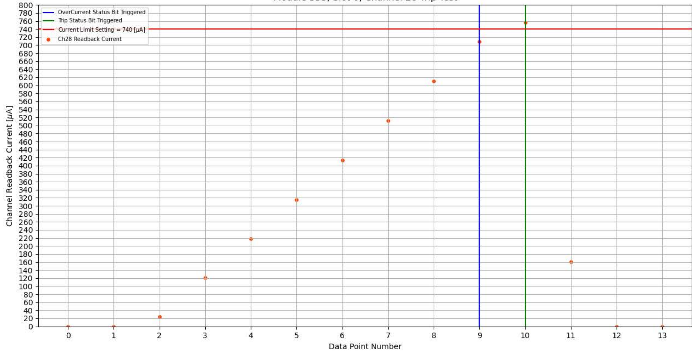
Module 353, Slot 0, Channel 28 Trip Test
