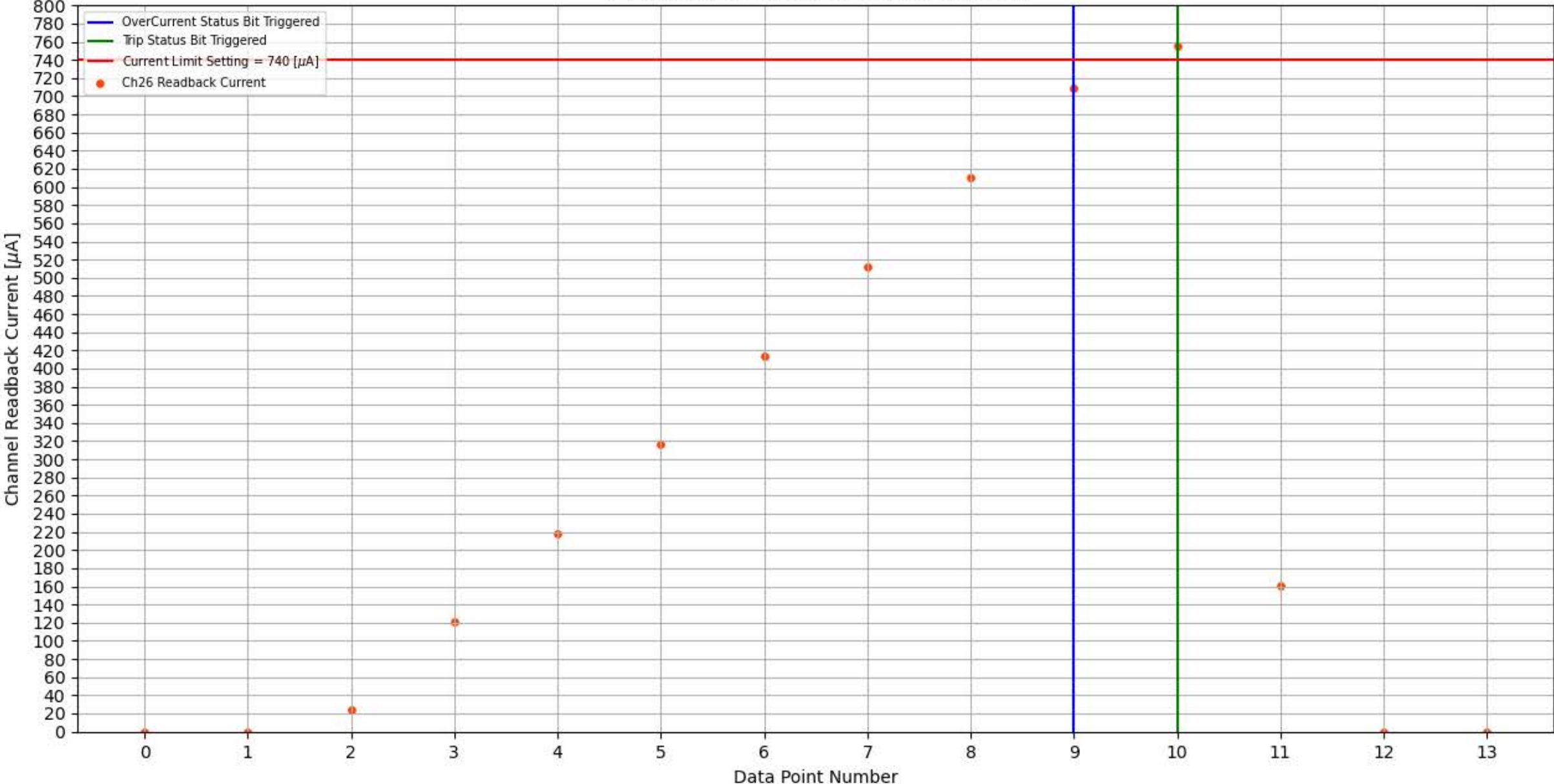
Module 353, Slot 0, Channel 26 Trip Test
