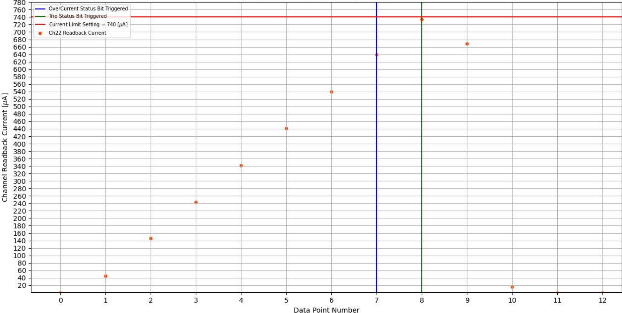
Module 353, Slot 0, Channel 22 Trip Test
