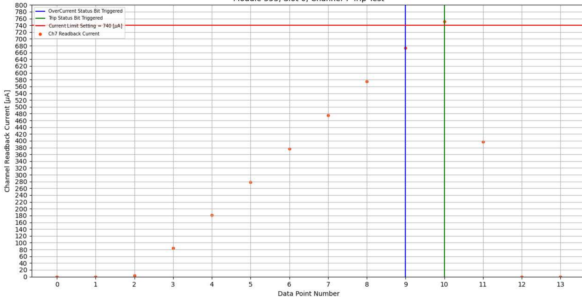
Module 353, Slot 0, Channel 7 Trip Test
