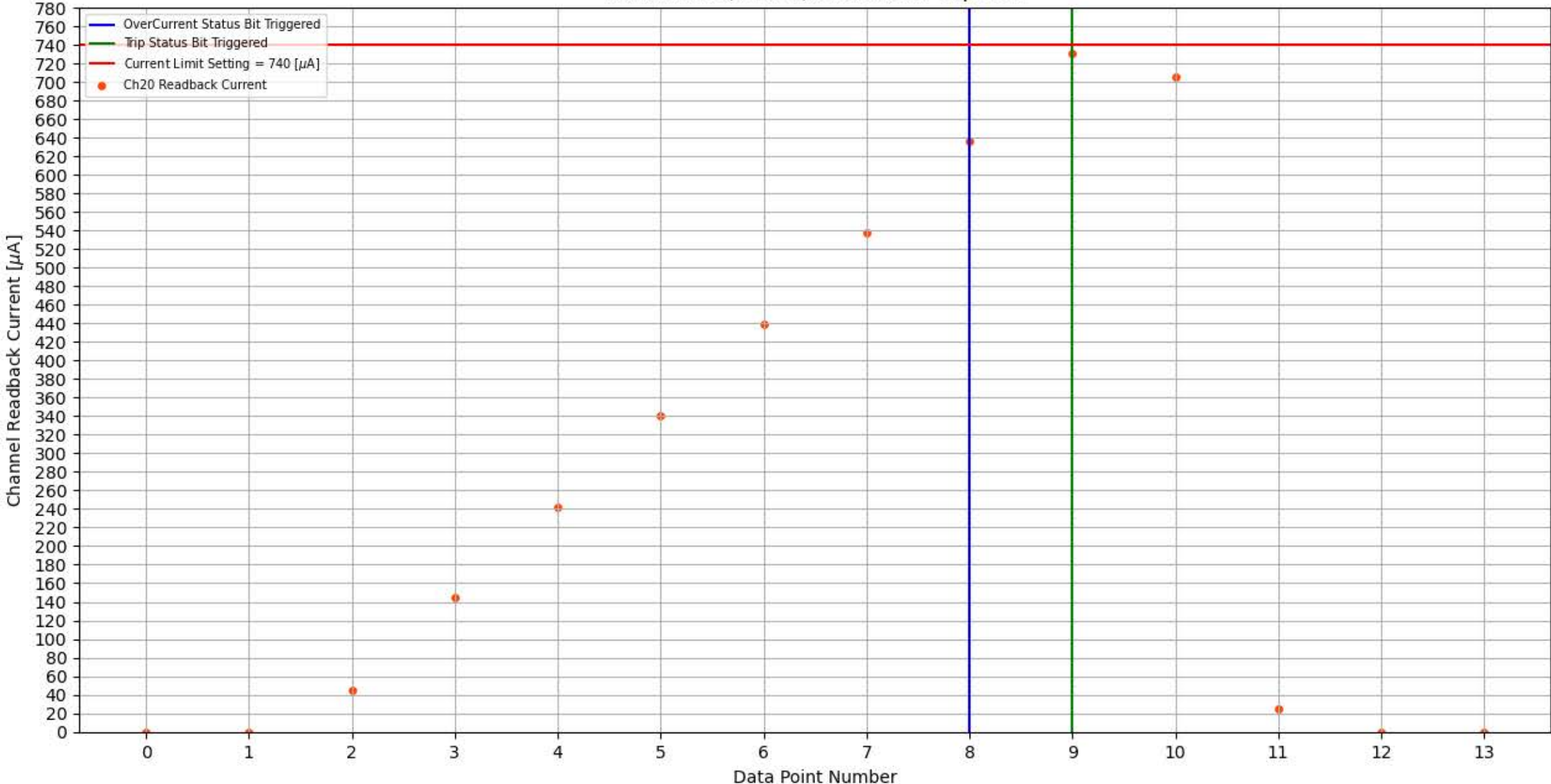
Module 353, Slot 0, Channel 20 Trip Test
