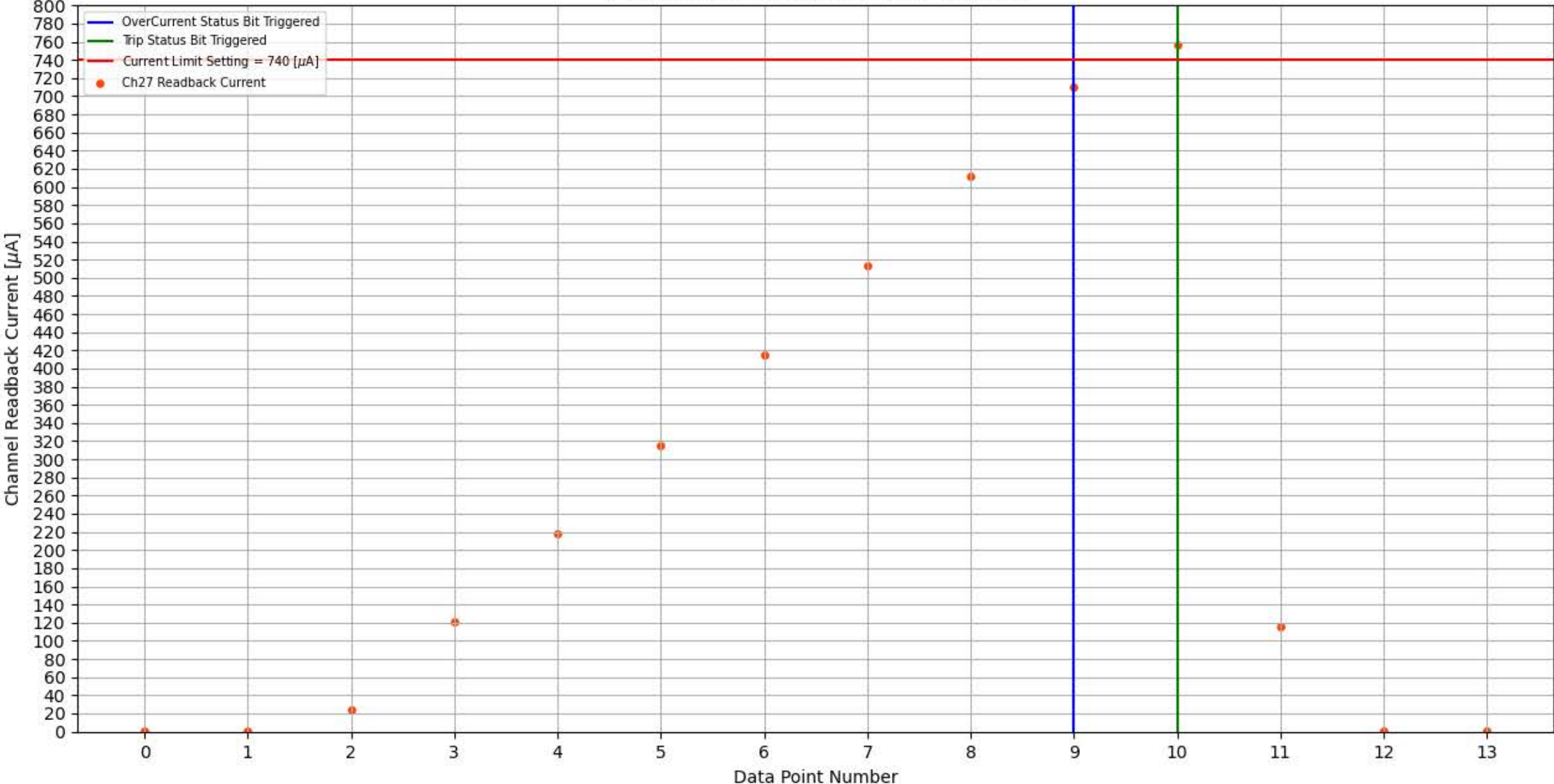
Module 353, Slot 0, Channel 27 Trip Test
