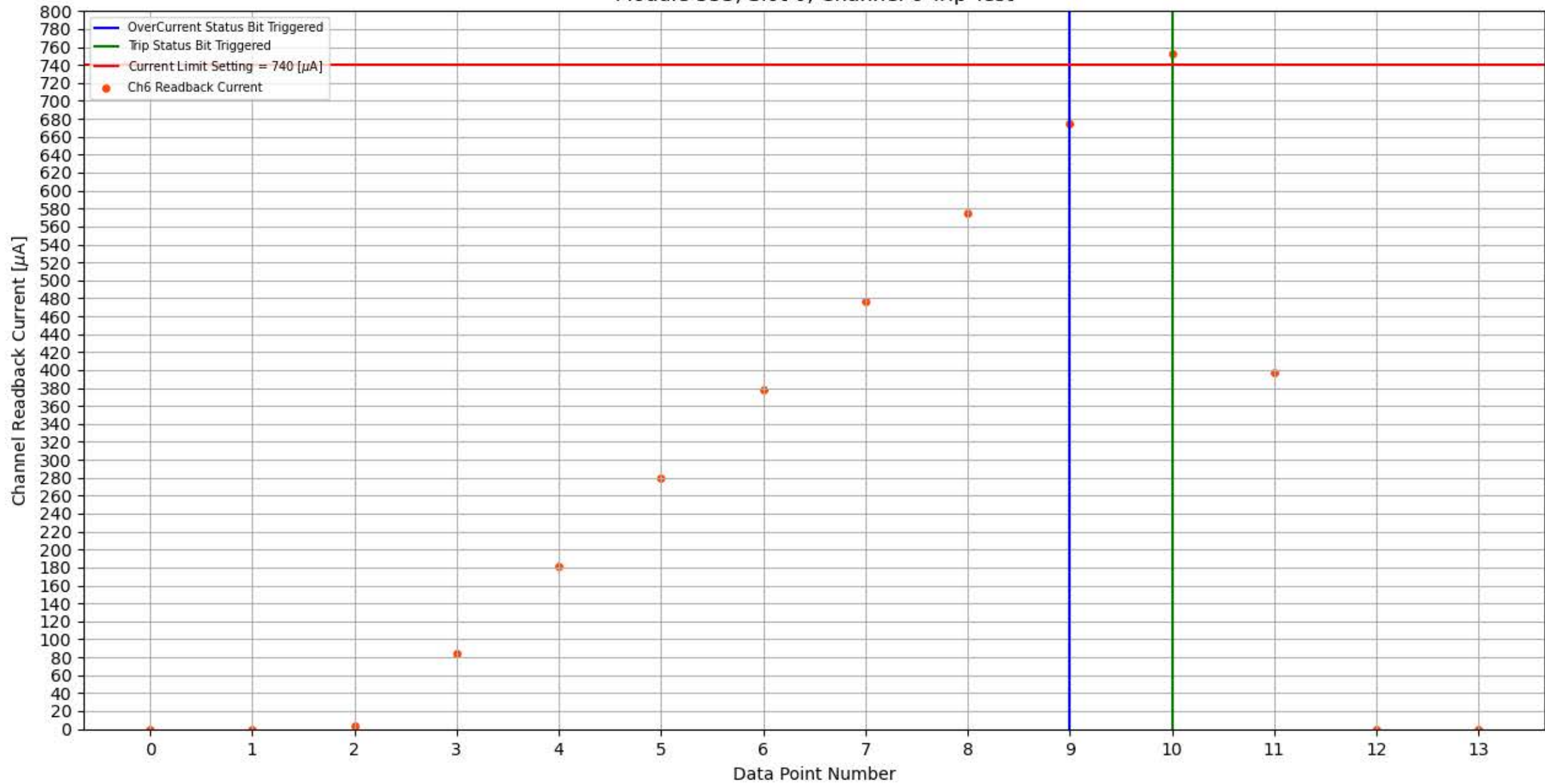
Module 353, Slot 0, Channel 6 Trip Test
