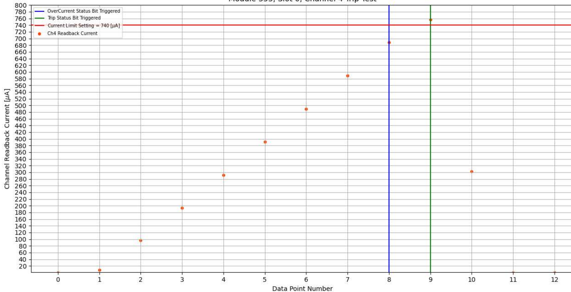
Module 353, Slot 0, Channel 4 Trip Test
