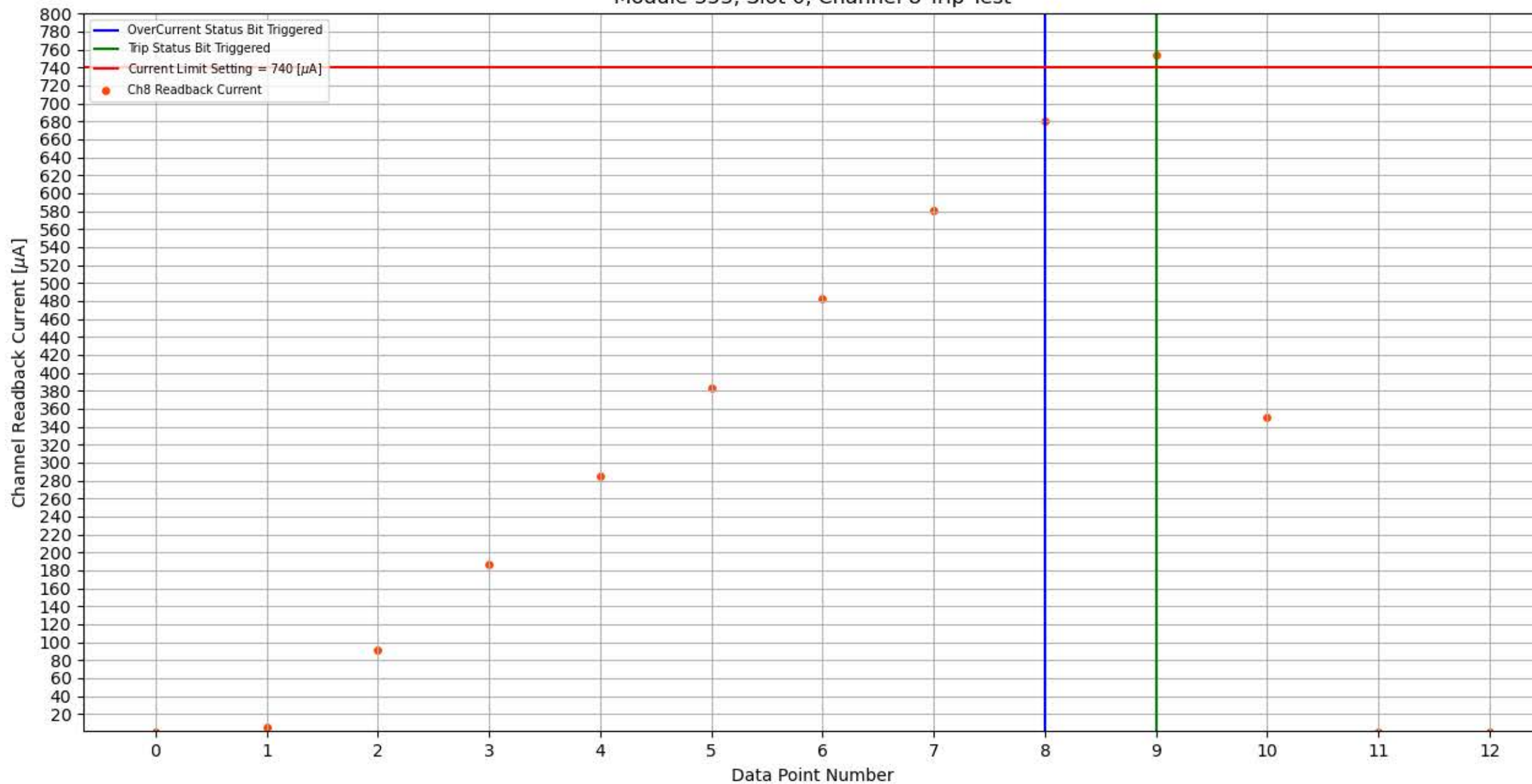
Module 353, Slot 0, Channel 8 Trip Test
