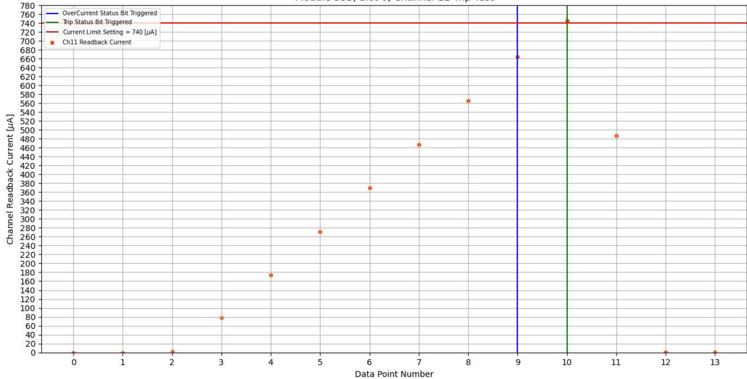
Module 353, Slot 0, Channel 11 Trip Test
