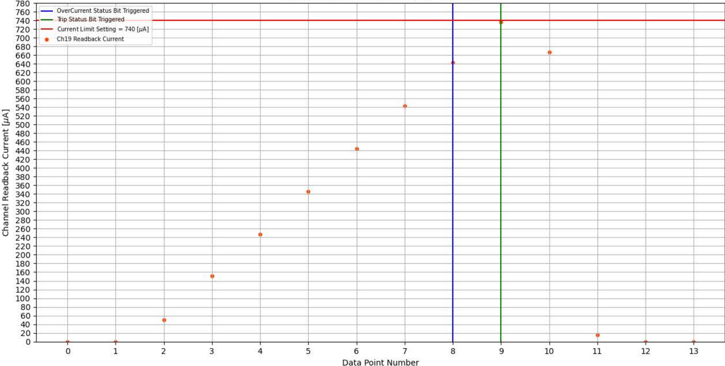
Module 353, Slot 0, Channel 19 Trip Test
