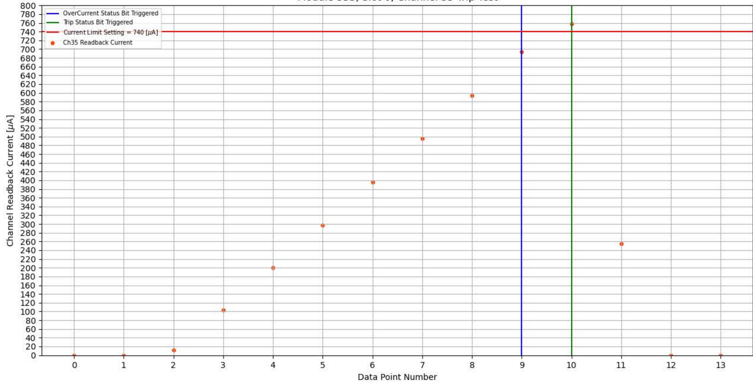
Module 353, Slot 0, Channel 35 Trip Test
