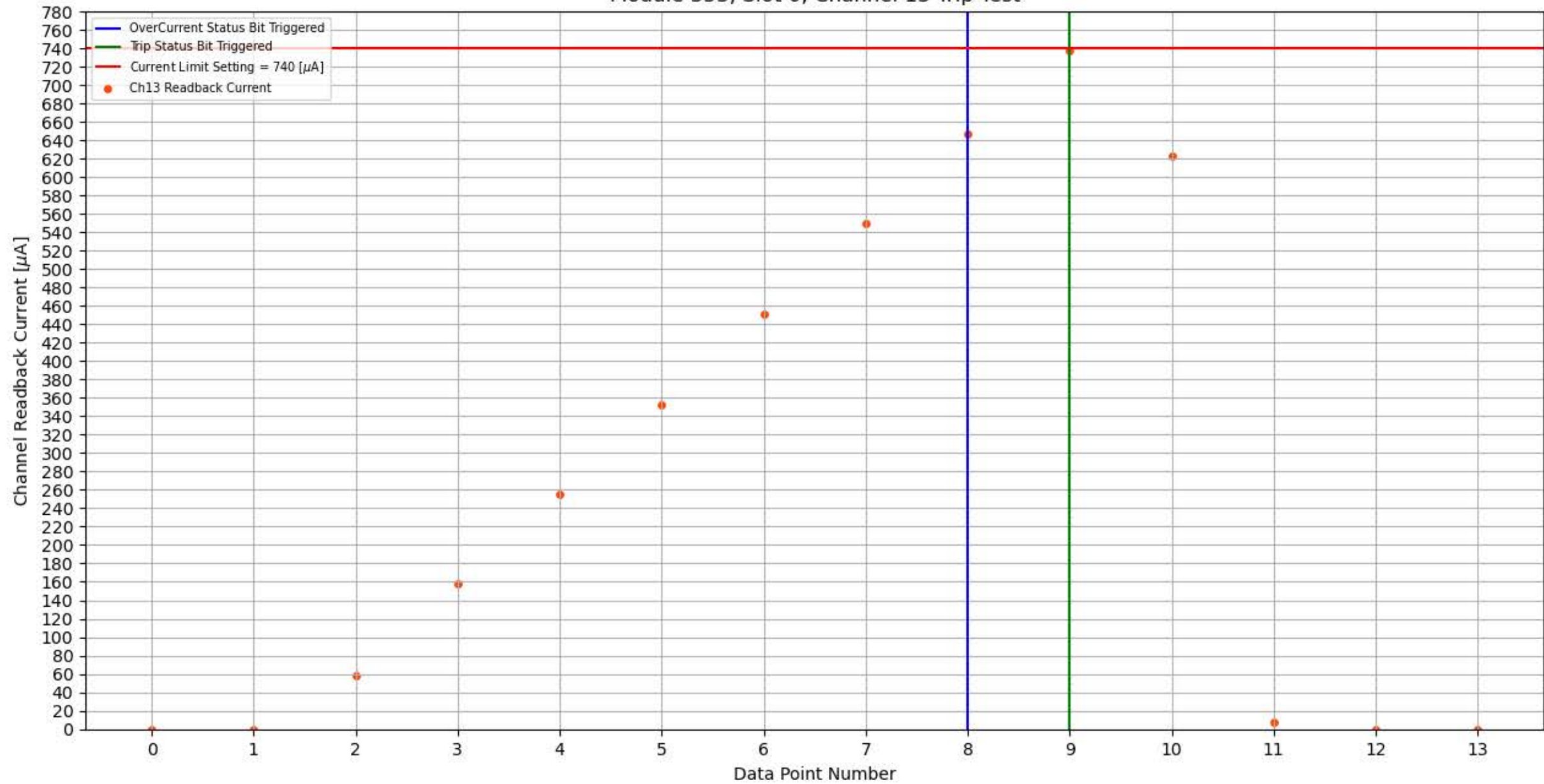
Module 353, Slot 0, Channel 13 Trip Test
