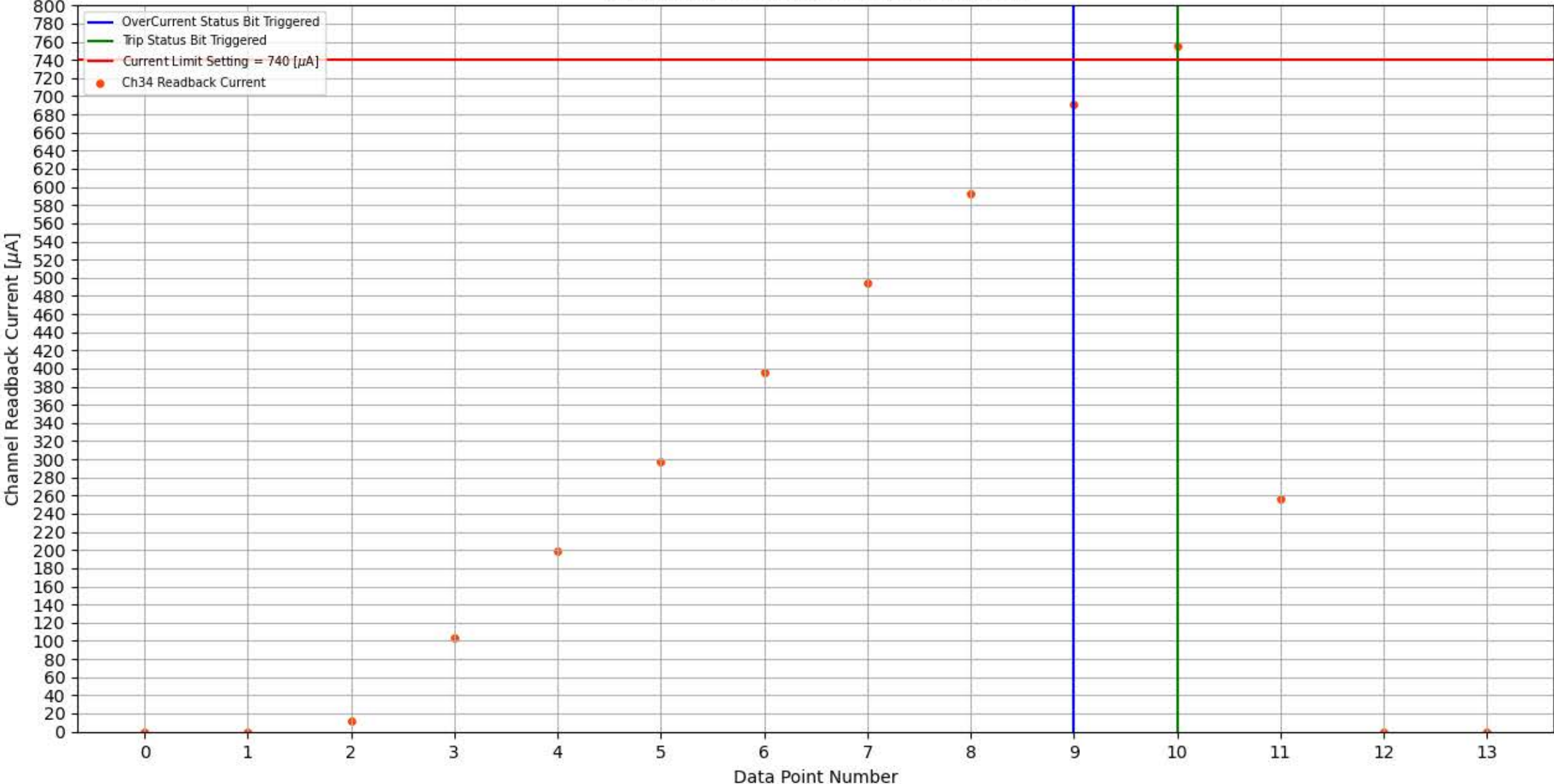
Module 353, Slot 0, Channel 34 Trip Test
