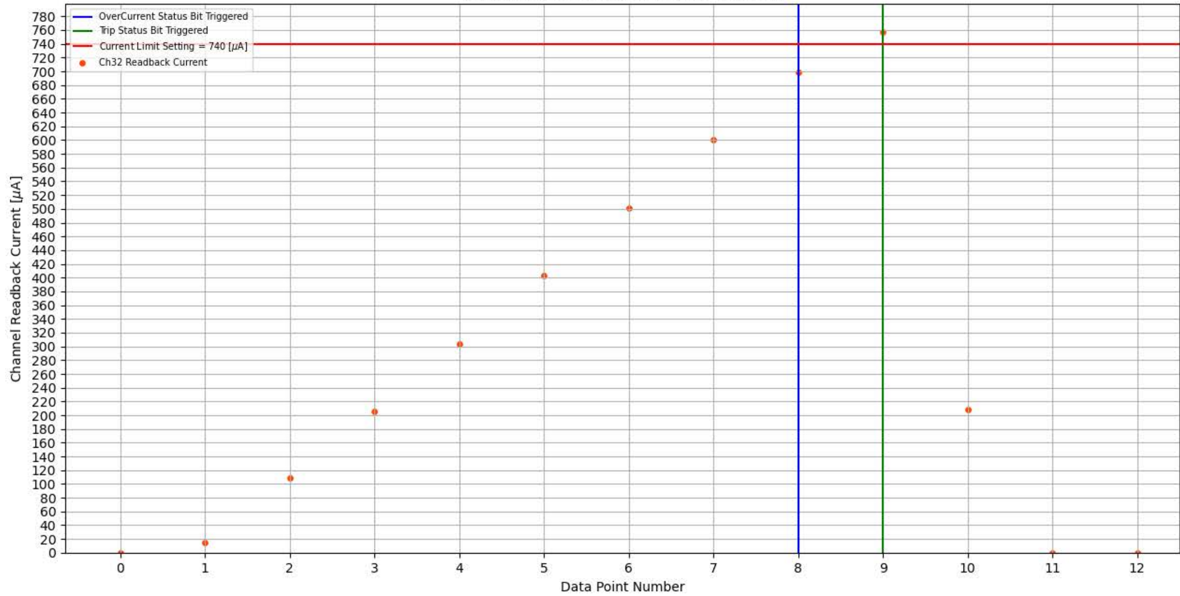
Module 353, Slot 0, Channel 32 Trip Test
