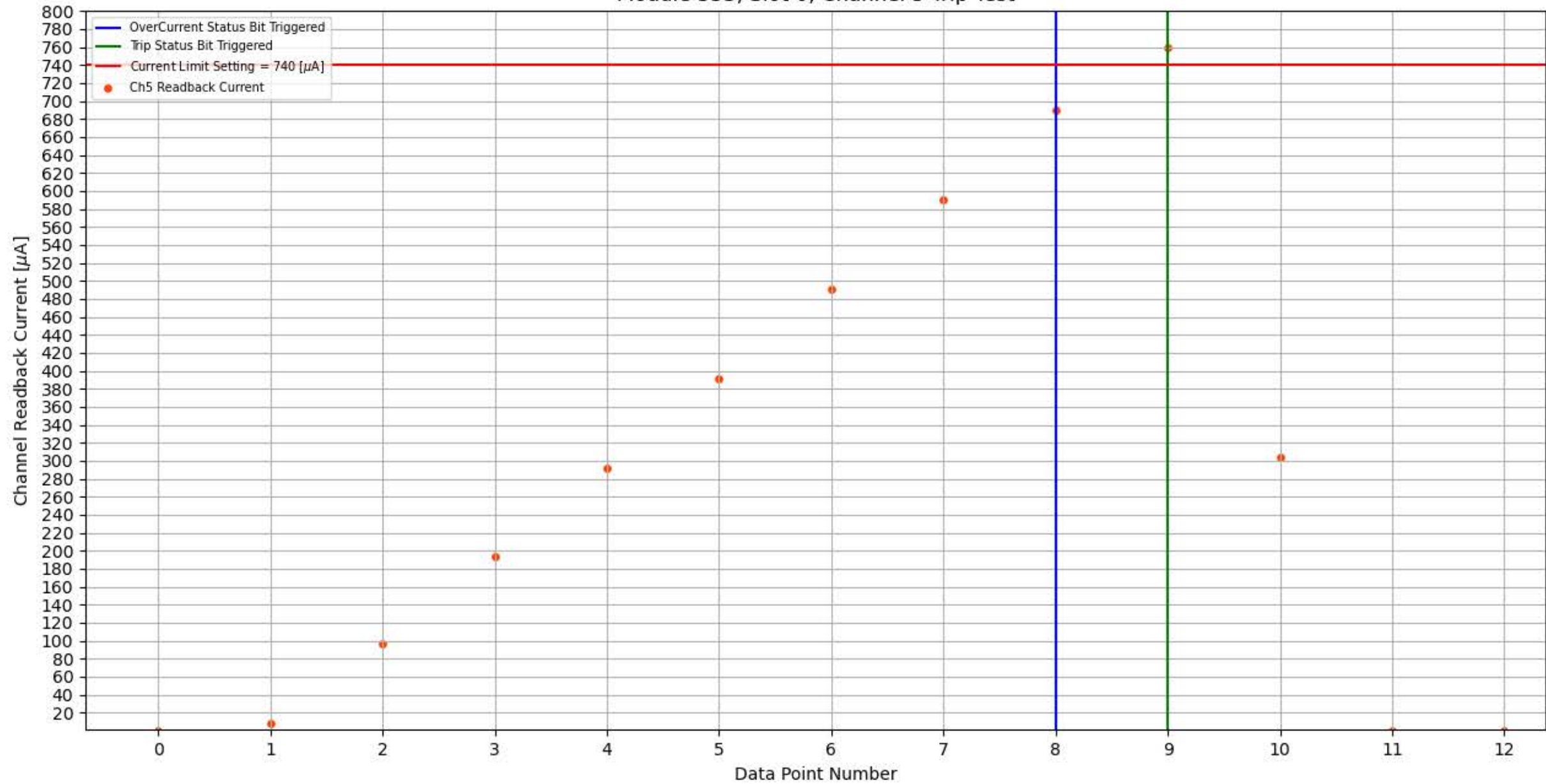
Module 353, Slot 0, Channel 5 Trip Test
