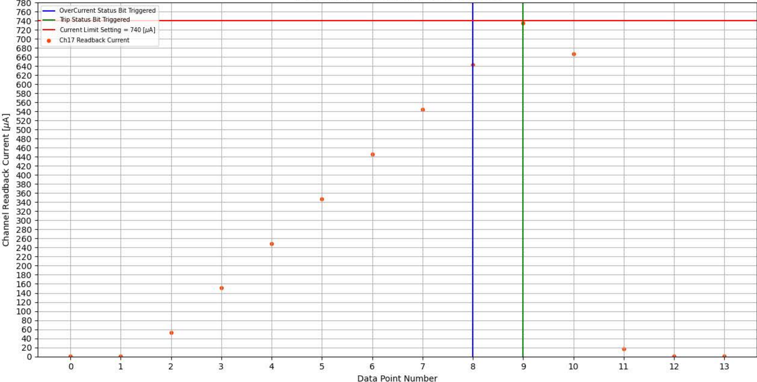
Module 353, Slot 0, Channel 17 Trip Test
