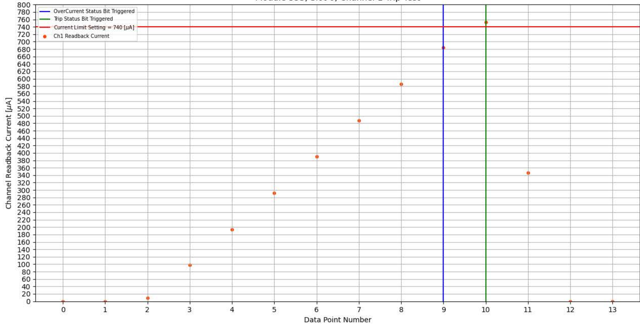
Module 353, Slot 0, Channel 1 Trip Test
