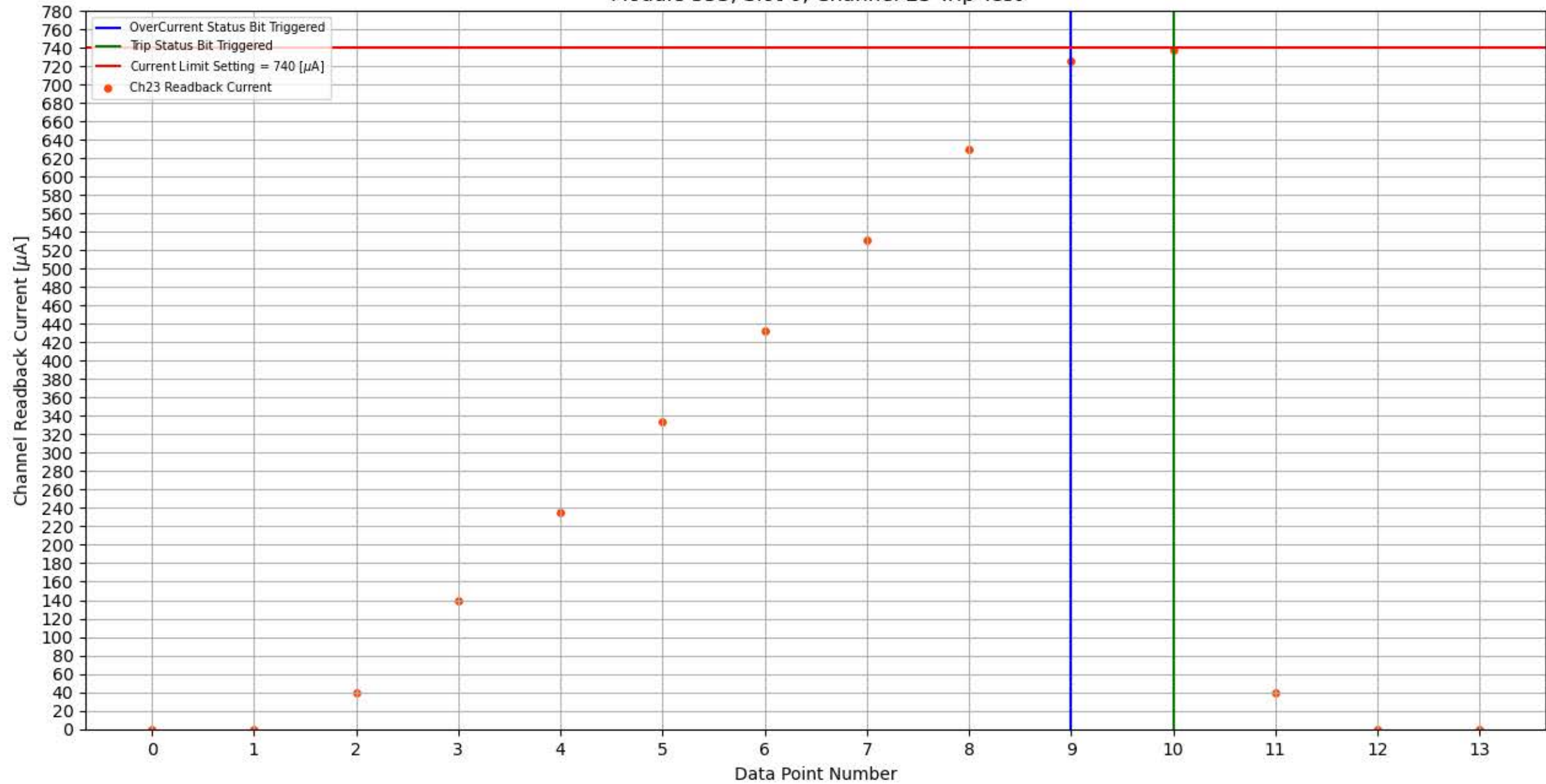
Module 353, Slot 0, Channel 23 Trip Test
