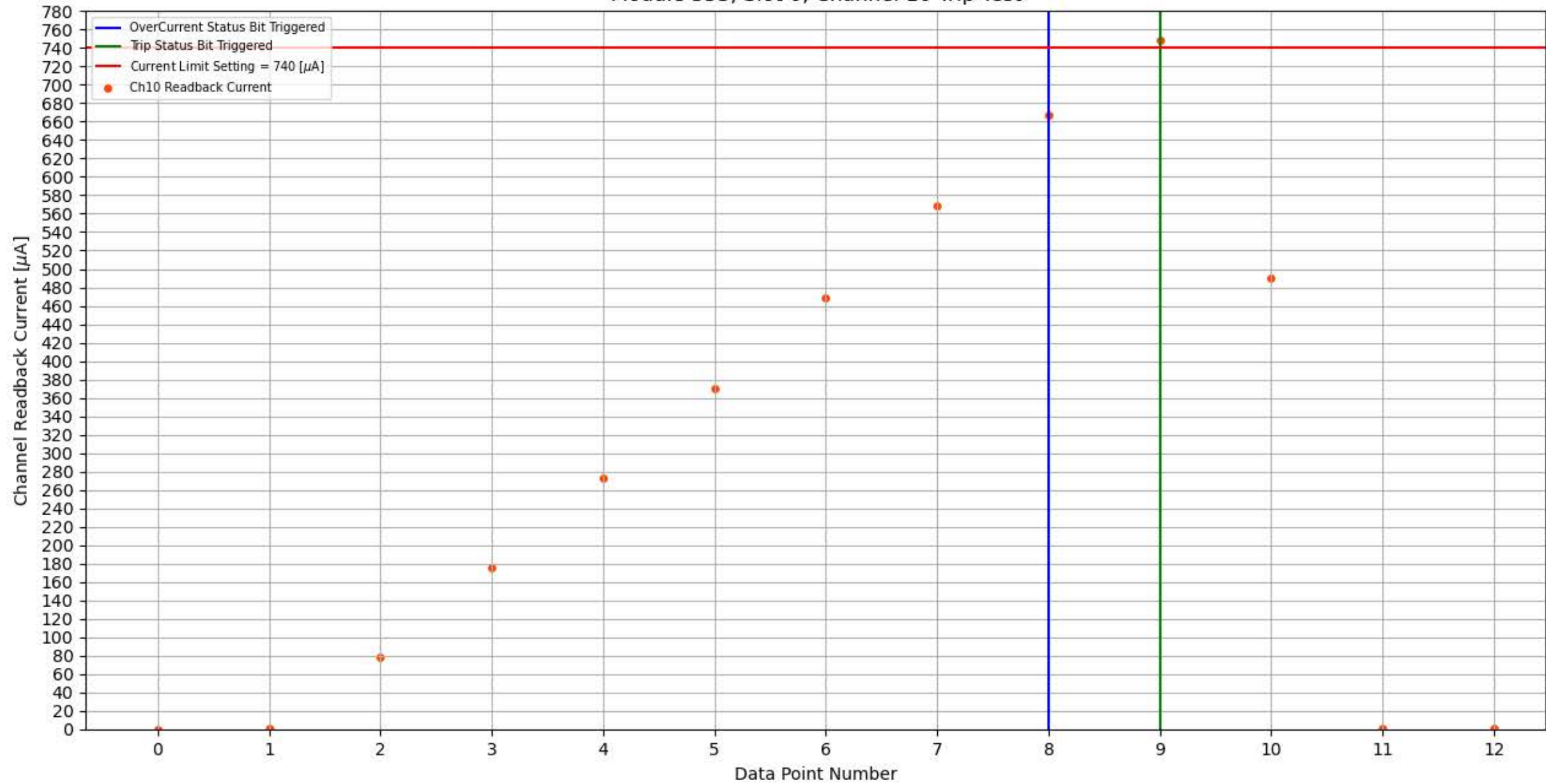
Module 353, Slot 0, Channel 10 Trip Test
