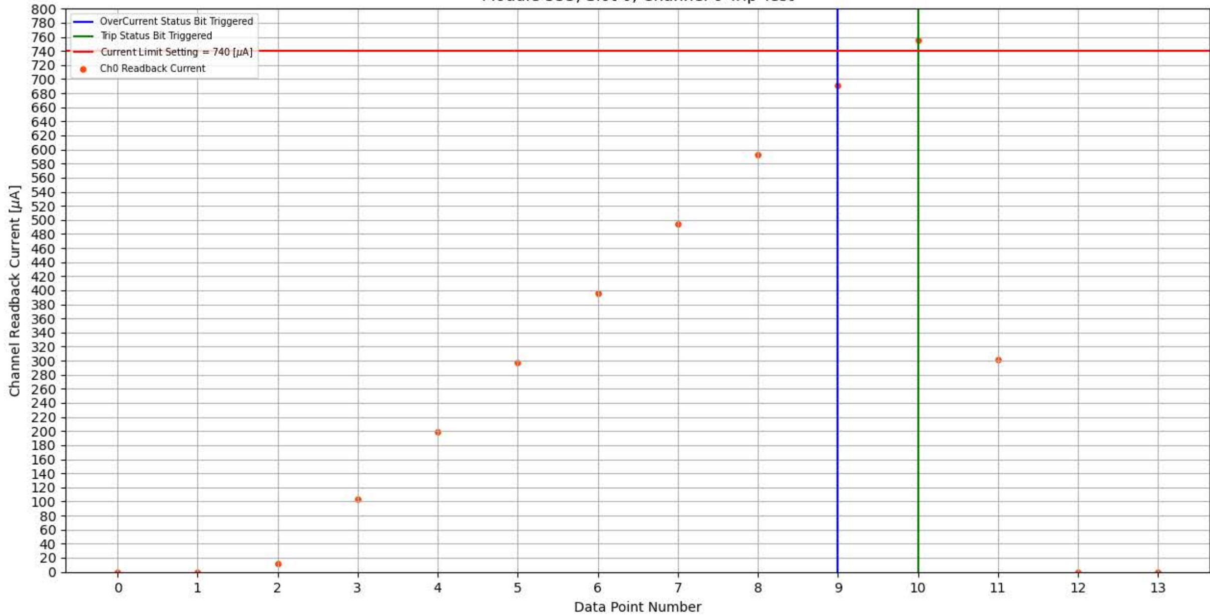
Module 353, Slot 0, Channel 0 Trip Test
