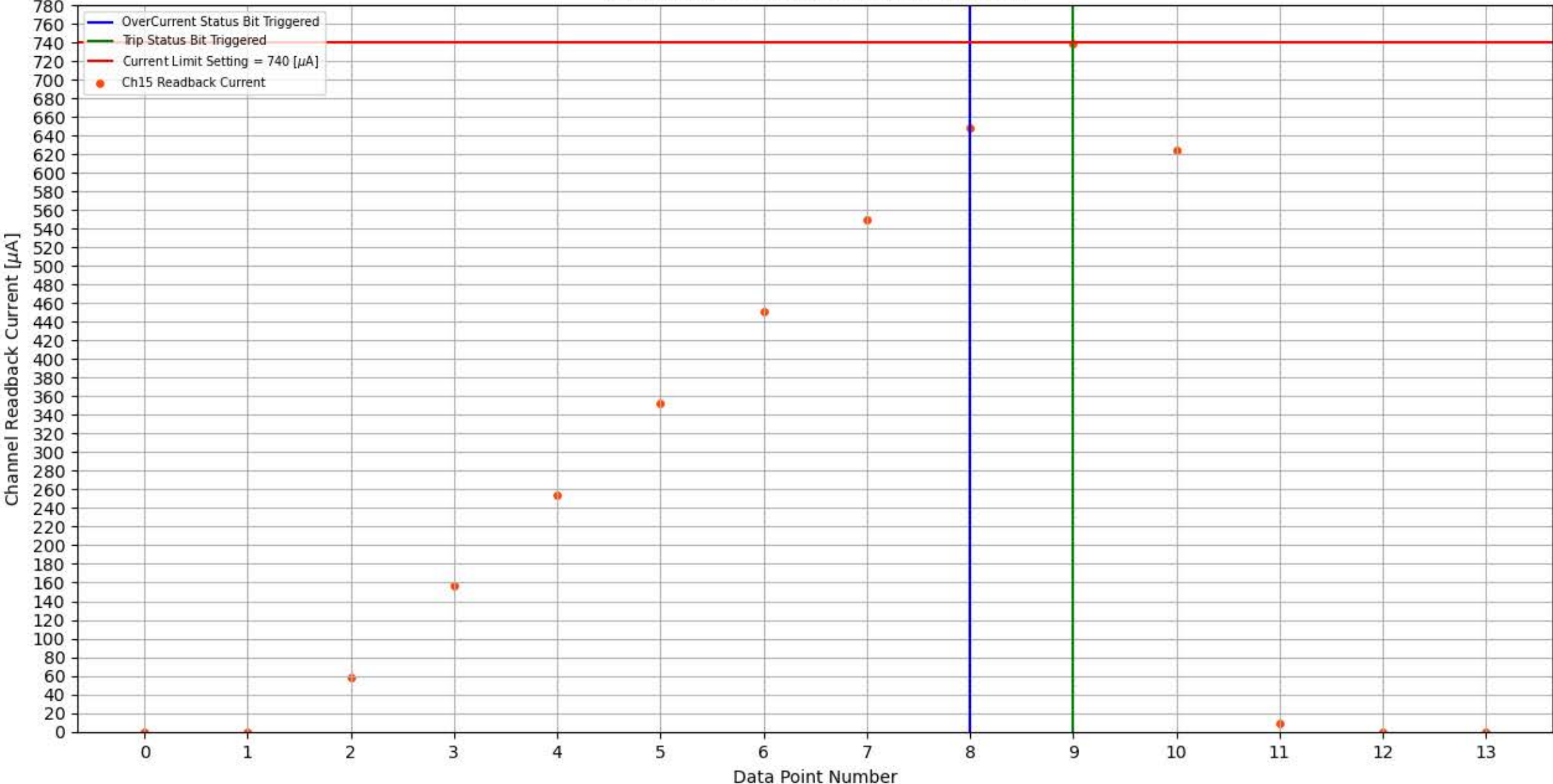
Module 353, Slot 0, Channel 15 Trip Test
