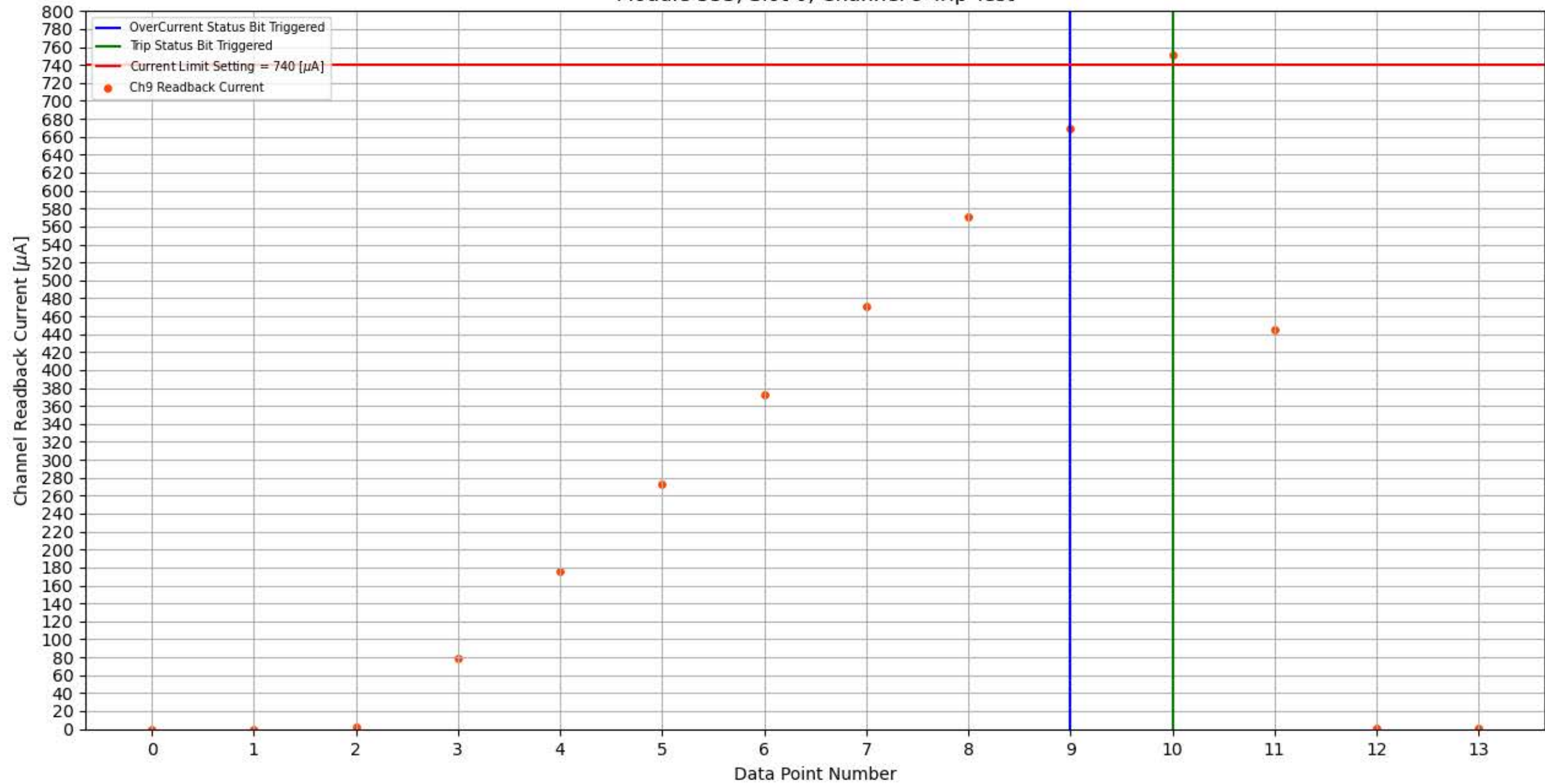
Module 353, Slot 0, Channel 9 Trip Test
