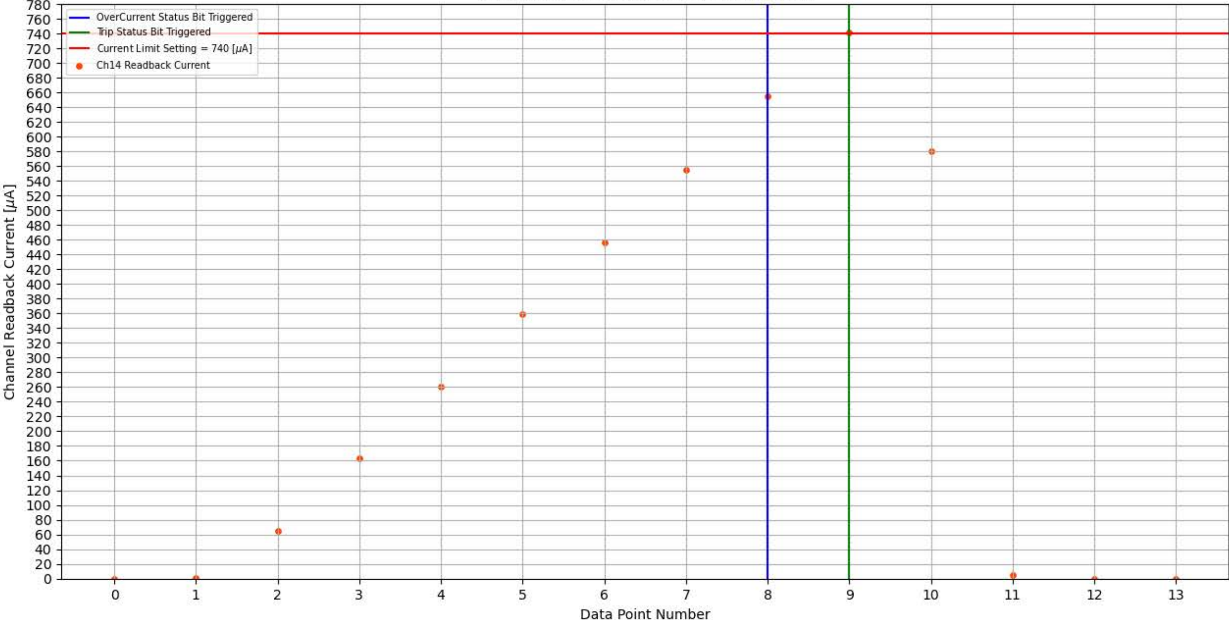
Module 353, Slot 0, Channel 14 Trip Test
