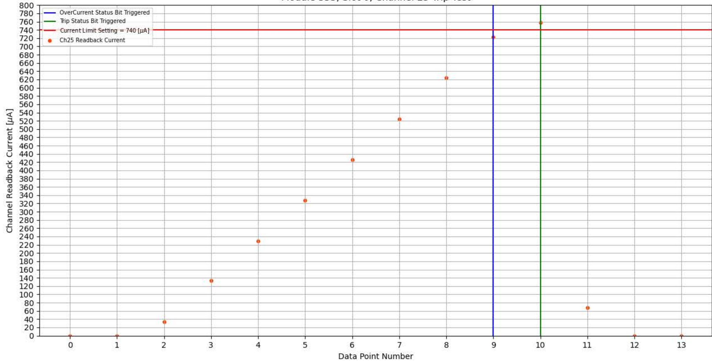
Module 353, Slot 0, Channel 25 Trip Test
