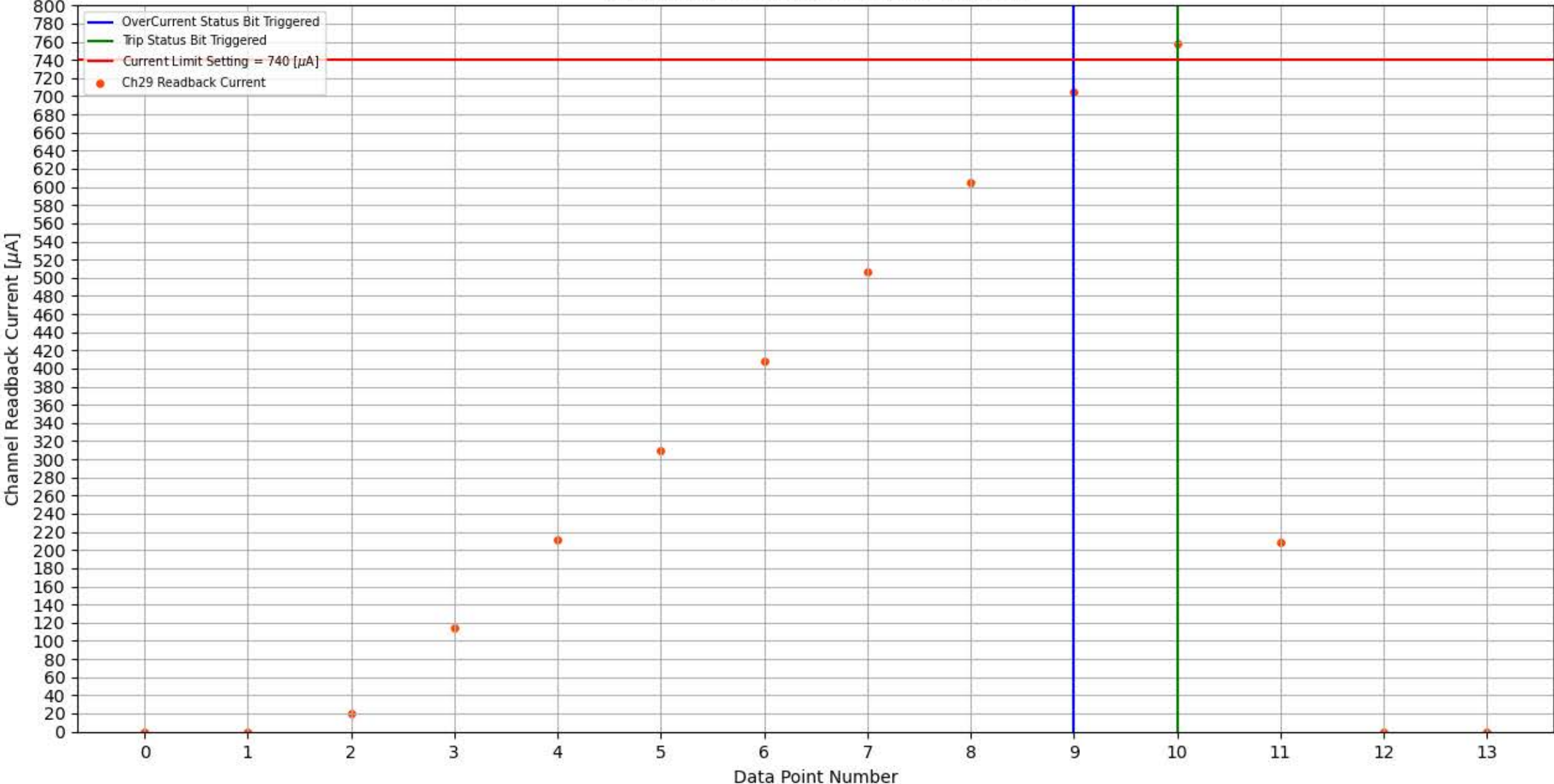
Module 353, Slot 0, Channel 29 Trip Test
