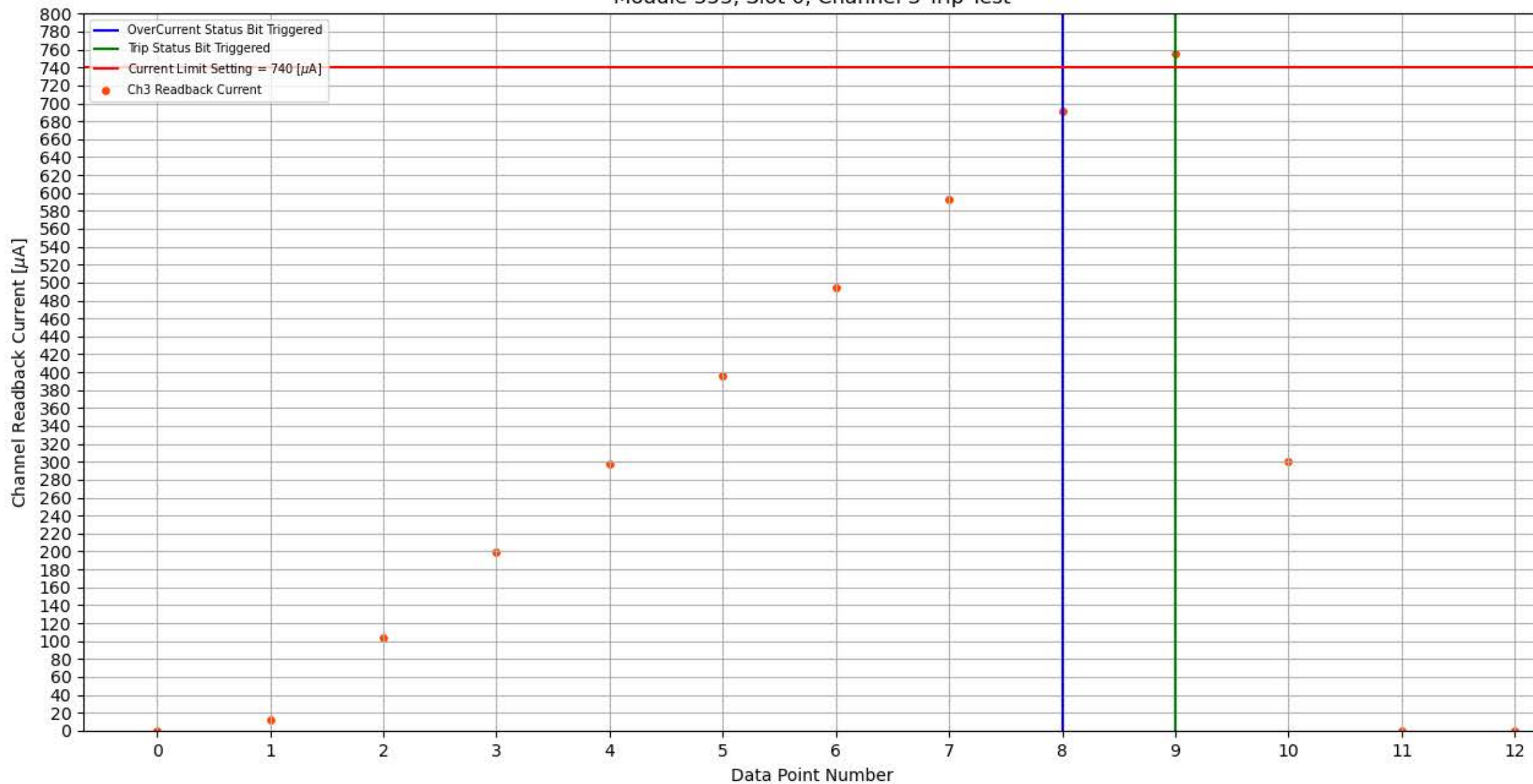
Module 353, Slot 0, Channel 3 Trip Test
